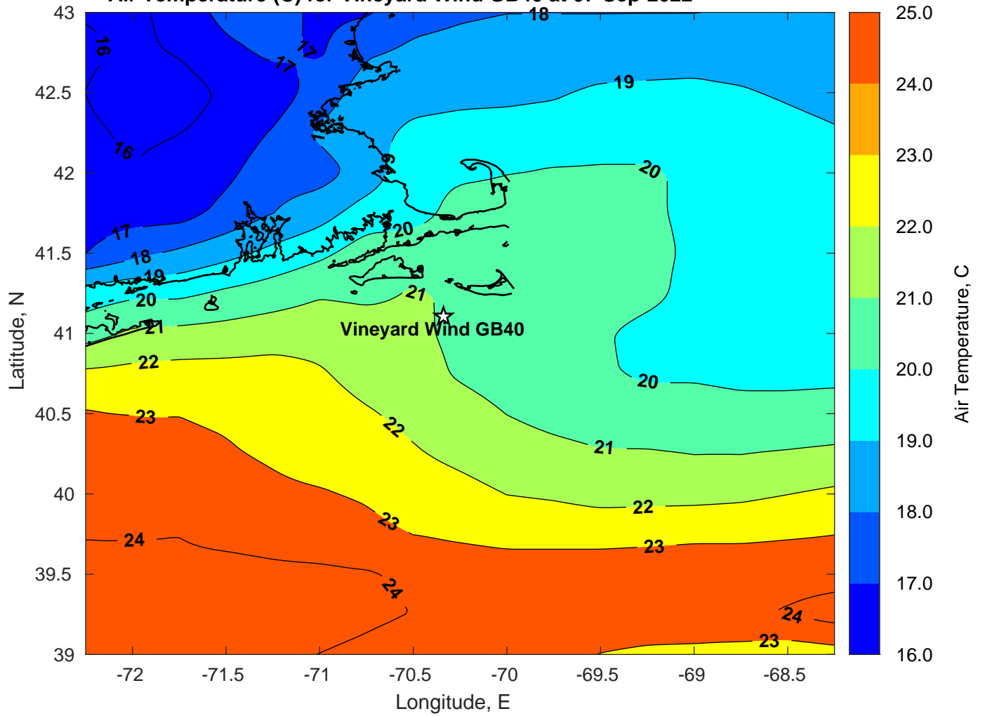
Air Temperature (C) for Vineyard Wind GB40 at 07-Sep-2022
